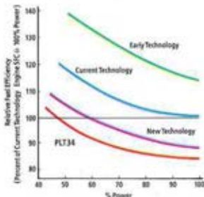
Relative Fuel Efficiency of Smaller Class Turboshaft Engines
